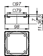
Opzetstuk DalIDrain Individual
