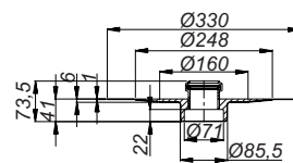
Brandwerendelement 12
